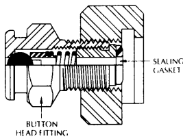
AUX 1200 Standard Type
