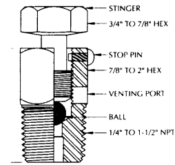
7834 (1/2" NPT) Standard Hex Head Style For Service to 10,000 PSI
