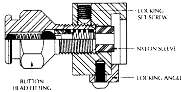
AUX 1200-LO Nylon Insert / Lock-On Style
