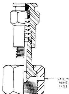
1714 with Giant Button Head & Ball Check Available w/ 1" - 14 THD WKM/API 7/8" - 14 THD McEvoy 3/4" - 16 THD Cameron
