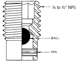
CV-14 (1/4" NPS) Single Ball (Floating) For Service to 10,000 PSI
